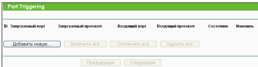
Рис. 4-34 Port Triggering
